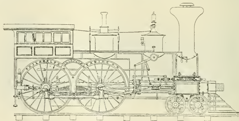
MILLHOLLAND'S FIRST PASSENGER ENGINE. FIG. 76.
